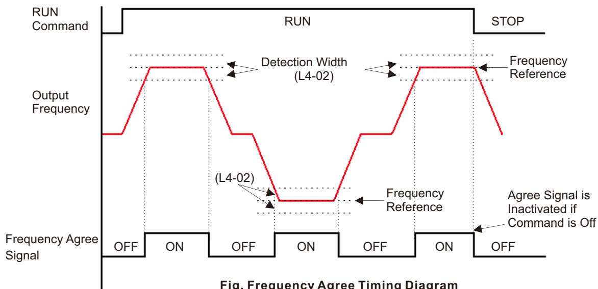
Fig. Frequency Agree Timing Diagram
