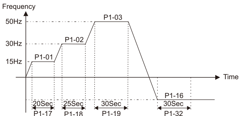
Fig. Executes 1 Cycle Operation then Keep Running at Last Process Speed (P1-00= 3 or 6)
