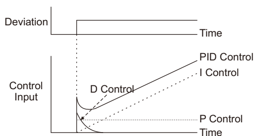
Fig. PID Operation
