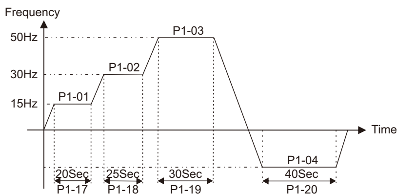
Fig. Executes 1 Cycle Operation then Stop (P1-00= 1 or 4)
