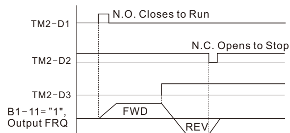
Fig. Terminal Signal Timing Sequence
