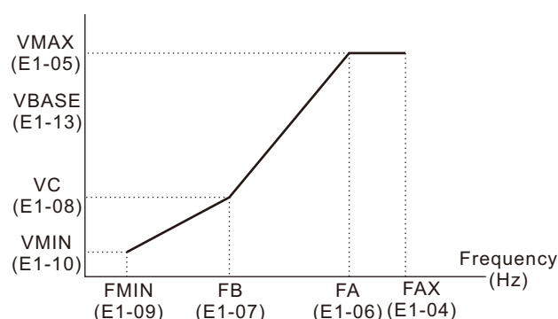
Fig. Custom V/F Pattern
