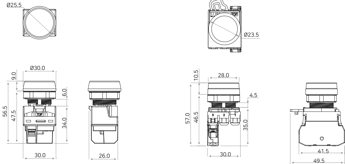
Push Button
