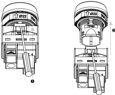
Pilot Light
